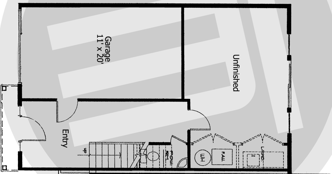
basement
