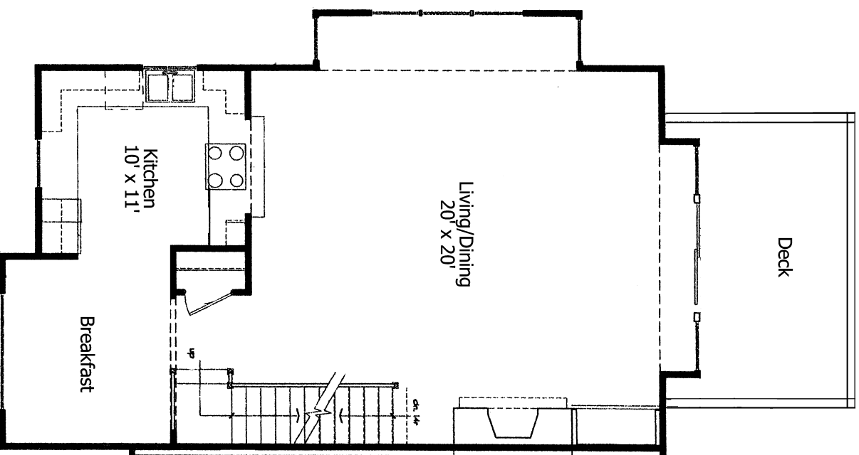
1st floor
