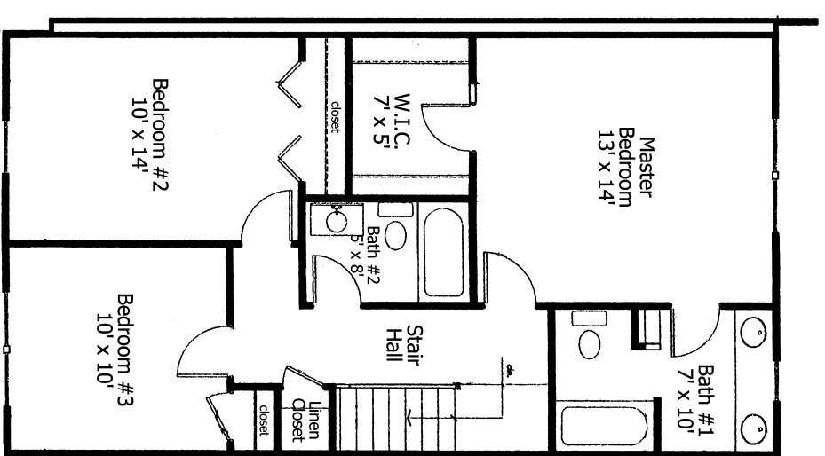
2nd floor
